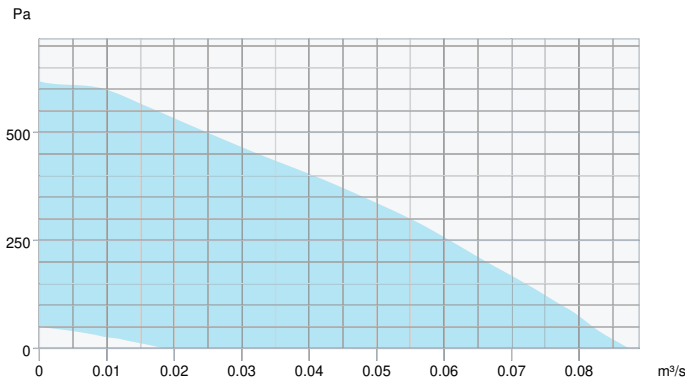
Supply - Performance curve
